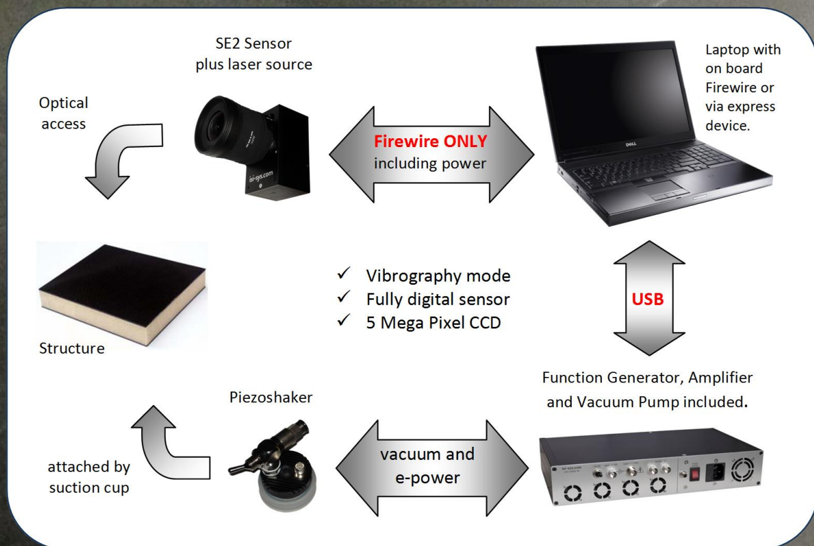
SE2 Sensor with full digital system concept
